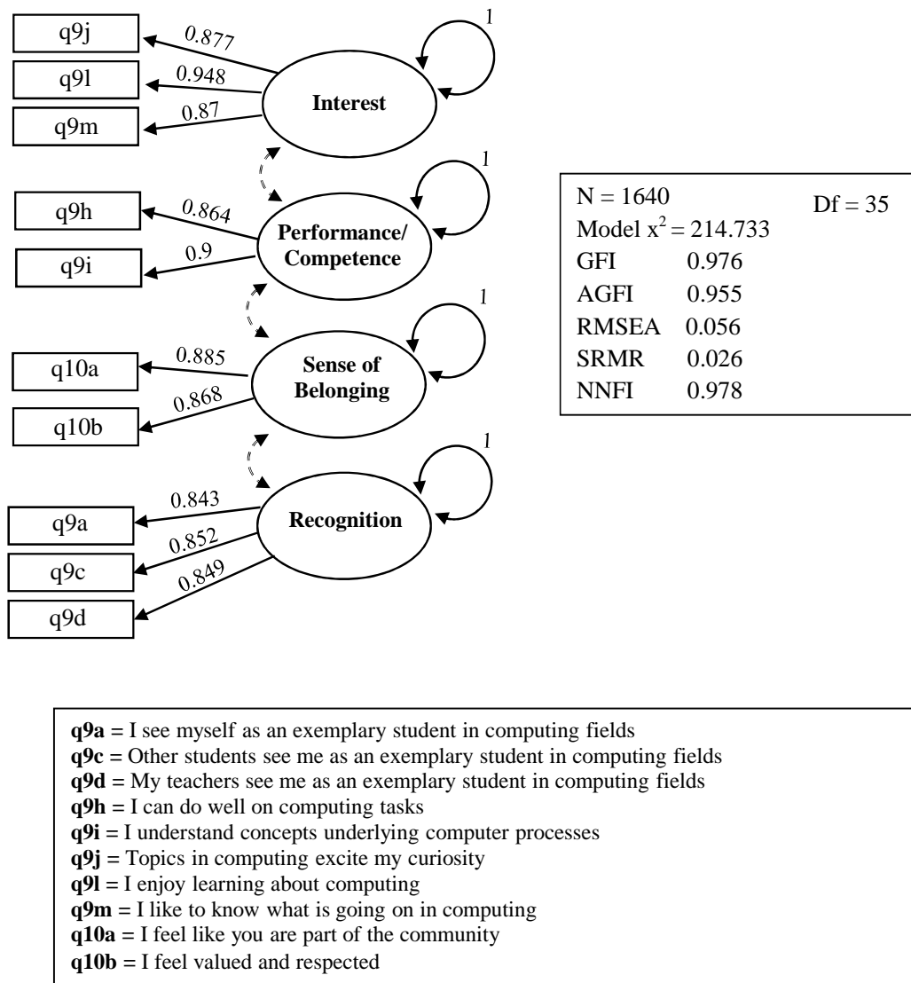
Fig. 2. Confirmatory factor analysis to confirm the factorial structures. (Acceptable values: GFI ( p > 0.90 ), AGFI ( p > 0.90 ), RMSEA ( p < 0.08 ), NNFI ( p > 0.90 ), SRMR ( p < 0.08 ))
